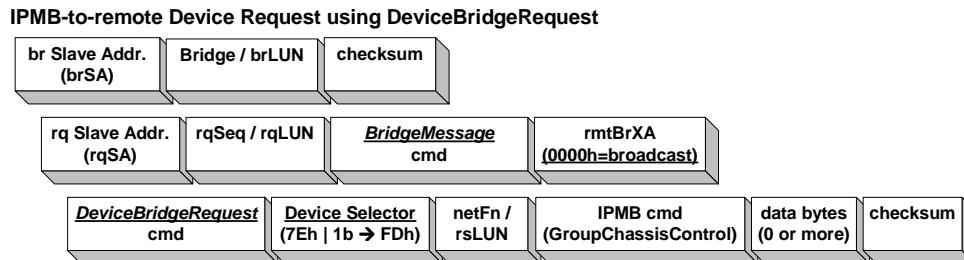
Figure 3-9, IPMB to Remote Device Request Format
