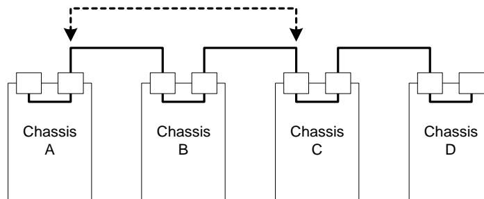
Figure 4-9, Daisy-chain Interconnect
