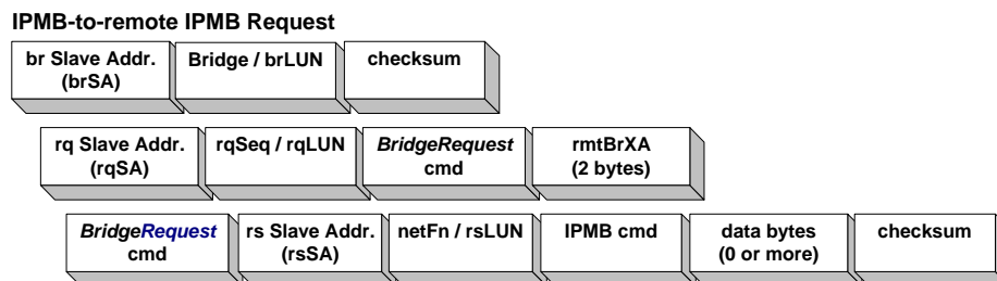
Figure 3-7, Full IPMB-to-IPMB BridgeRequest Request Format
