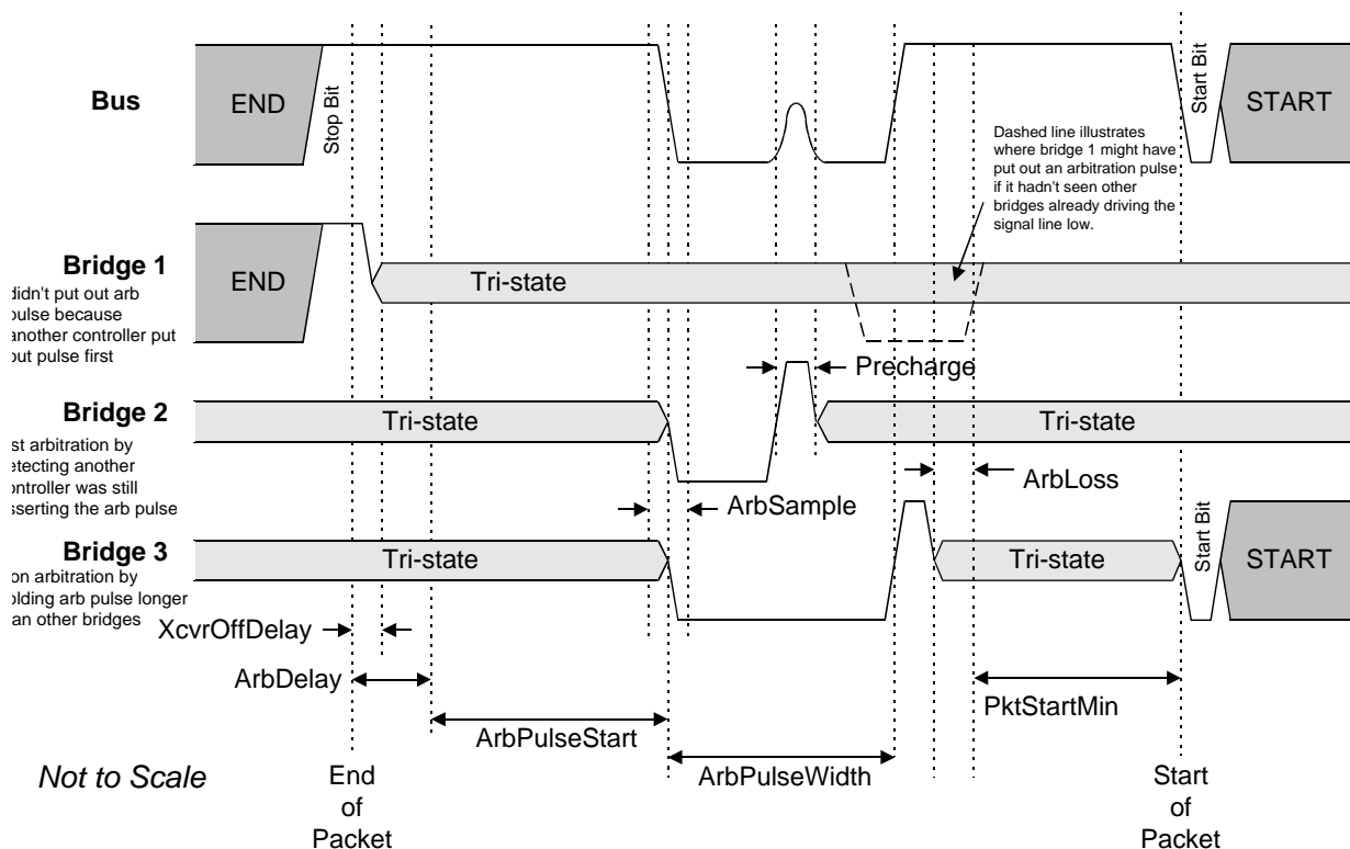
Figure 4-6, Arbitration Timing & Example
