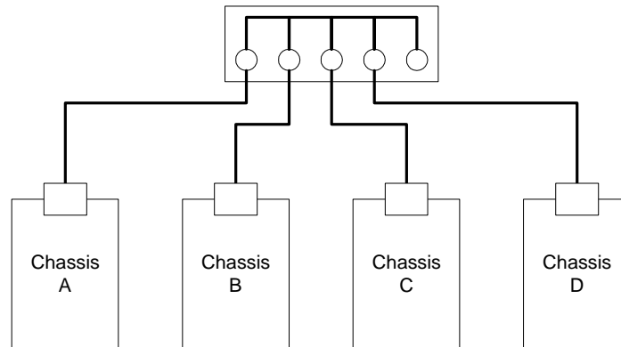
Figure 4-8, Passive Star Interconnect
